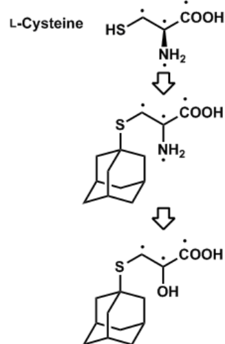
Figure 1. Incorporation of 13 C, 15 N-labeled (•) L-Cysteine
