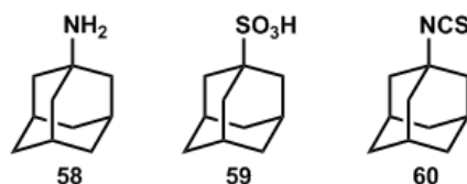
Figure 2. The structures of 1-aminoadamantane ( 58 ), 1-adamantanesulfonic acid ( 59 ) and isothiocyanic acid 1-adamantyl ester ( 60 )
