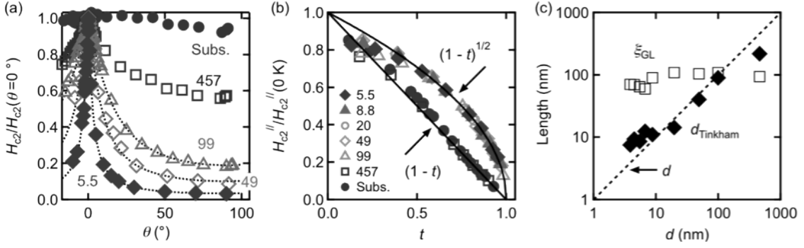
Fig. 4 (a) Normalized upper critical field H_{c2} vs angle \theta of the 1% samples with various thickness. Dotted lines are the fits using 2D superconductivity theory [3]. (b) Normalized parallel upper critical field H_{c2}^{\parallel} vs the reduced temperature t = T/T_c . Solid lines are the theory curves. (c) Ginzburg-Landau coherence length \xi_{GL} , and the thickness of superconducting layer d_{Tinkham} plotted with d .
