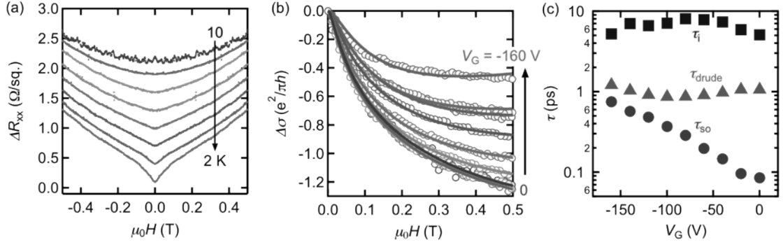
Fig. 6 (a) Magnetoresistance of a 1 at. % sample ( d = 3.9 nm) at low temperatures. (b) Gate voltage ( V_G ) dependence of weak antilocalization correction to conductivity at T = 2 K. (c) Estimated inelastic scattering time \tau_i , SO scattering times \tau_{so} from the Hikami-Larkin-Nagaoka fits [6]. The Drude scattering times \tau_{drude} are estimated from Hall measurements.
