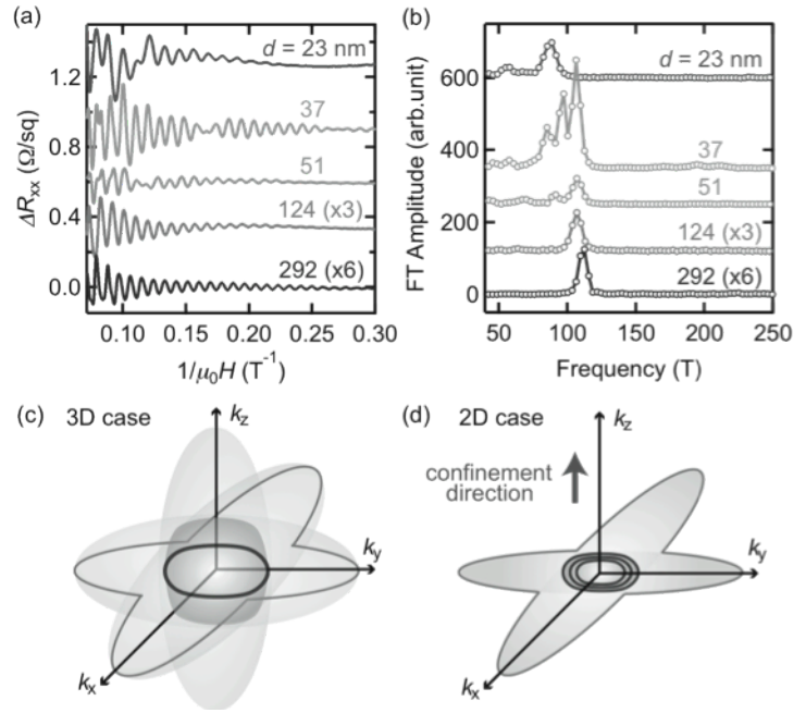
Fig. 2 (a) SdH oscillations measured at T = 100 mK in 0.2 at. % doped samples with various thickness d . (b) Fourier transformation (FT) spectra. (c,d) Schematic diagrams of the 3D and 2D Fermi surfaces based on the results.
