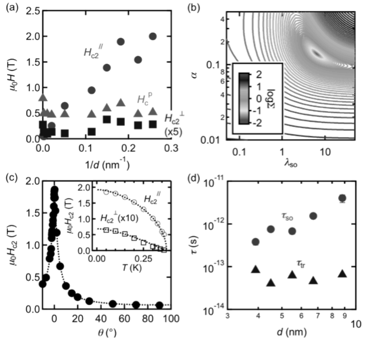
Fig. 5 (a) Upper critical field in the parallel geometry H_{c2}^{\parallel} , in the perpendicular geometry H_{c2}^{\perp} , and the Pauli limiting field H_c^p , plotted against 1/d . (b) Simulation result using the WHH theory [4]. \Sigma is [(\text{experimental data}) - (\text{theory})]^2 , \alpha is the orbital depairing parameter, and \lambda_{so} is the spin-orbit scattering rate. (c) Anisotropy and T dependence of H_{c2} of d = 5.5 nm sample. Dotted lines are the theory fit. (d) Spin-orbit scattering time \tau_{so} and momentum scattering time \tau_{tr} as a function of d .
