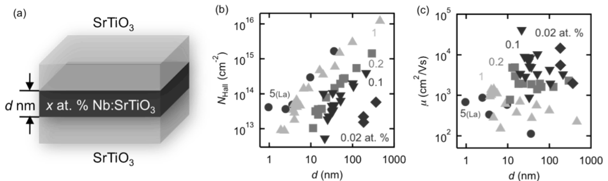
Fig. 1 (a) A schematic diagram of Nb \delta -doped SrTiO 3 heterostructures. (b) Sheet carrier density N_{\text{Hall}} , and (c) Hall mobility \mu estimated by the Hall measurement at temperature T = 2 K.
