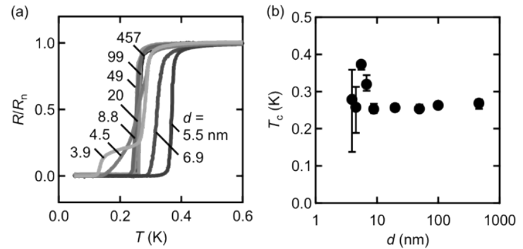
Fig. 3 (a) Normalized resistance plotted with temperature for 1 at. % doped samples with various thicknesses. (b) Superconducting transition temperature as a function of d . The error bar of data denotes the 10-90% width of the superconducting transition in (a).
