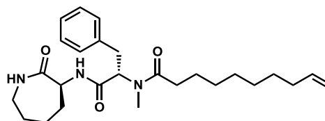
Ciliatamide A ( 10 )
