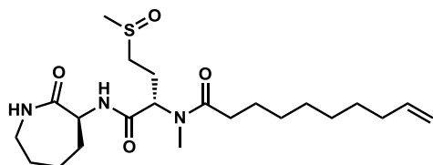
Ciliatamide D ( 9 )
